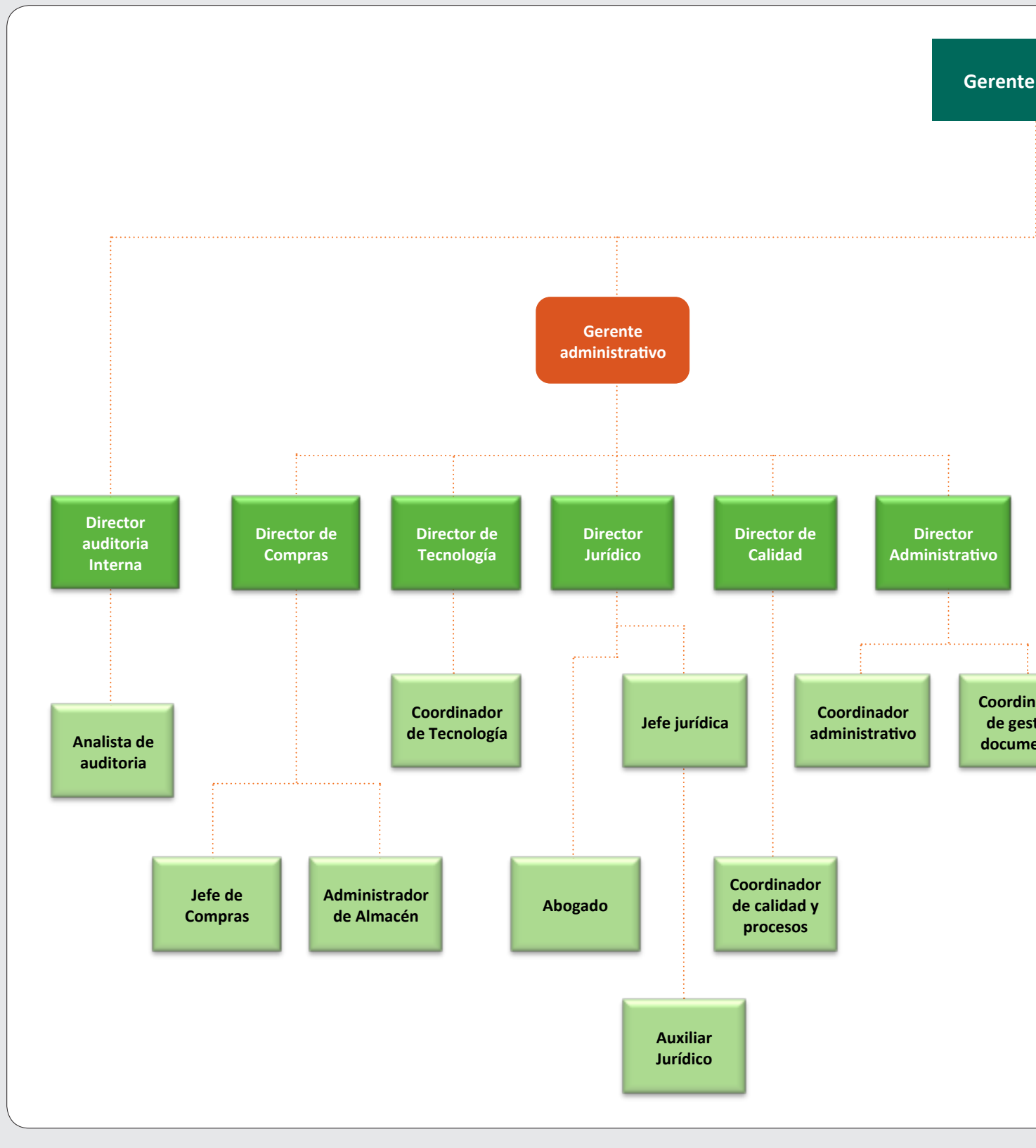
DIAGRAMA 2.1. ORGANIGRAMA
