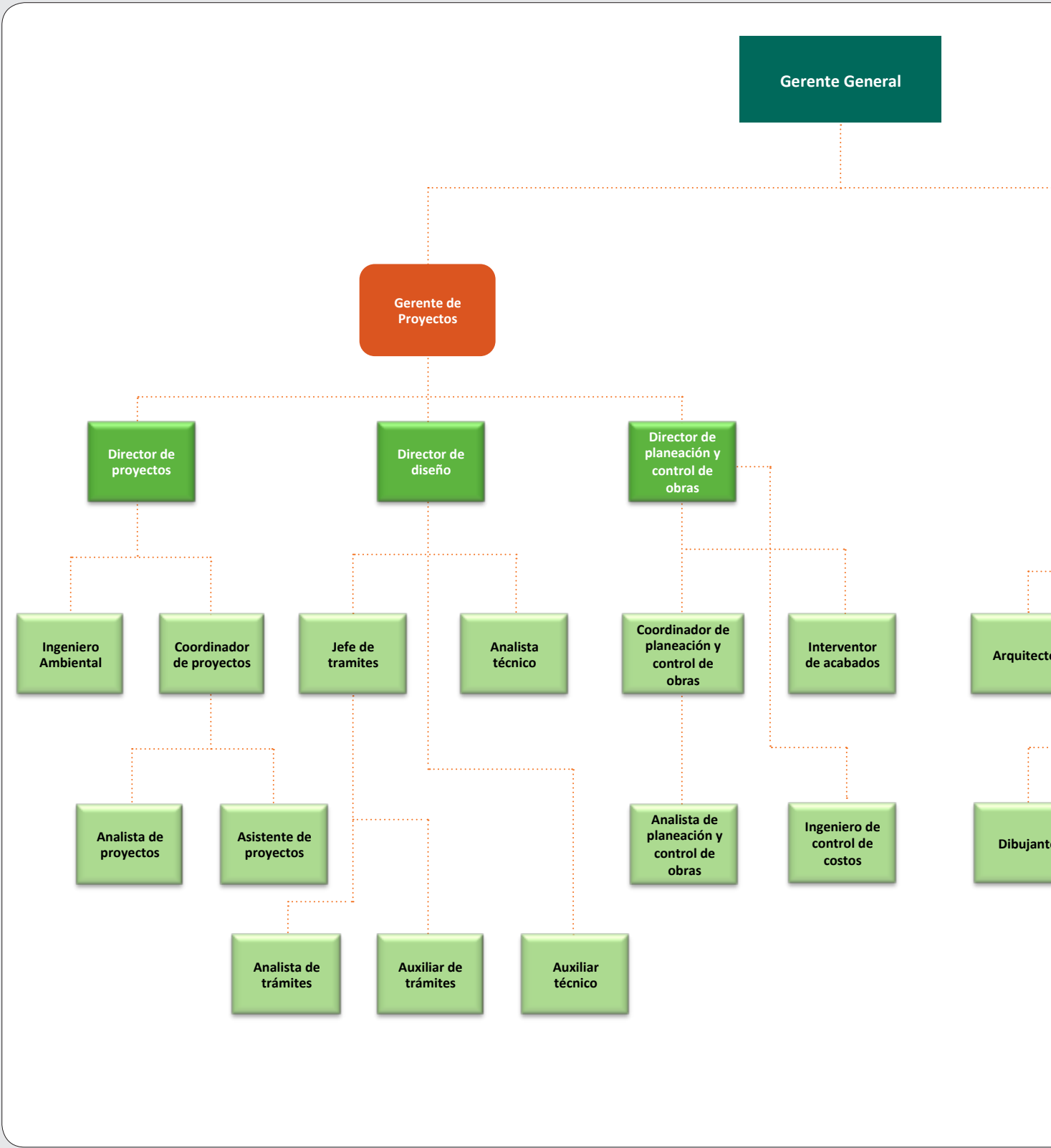
DIAGRAMA 2.2. ORGANIGRAMA
